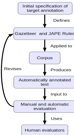
Fig. 1 - A Workflow Diagram
